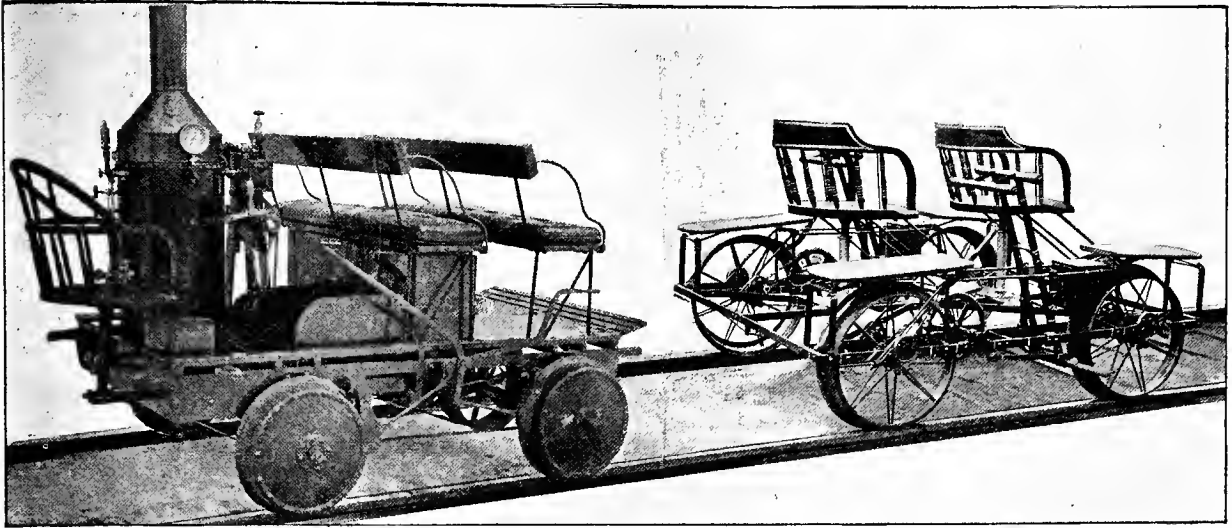
Fig. 5612 STEAM INSPECTION-CAR. Capacity, 7 persons. Weight, 1,000 lbs. Speed, 20 to 25 miles an hour.
